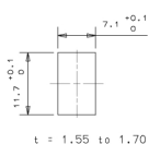
Figure 4 Cut-hole Dimensions for Reference
