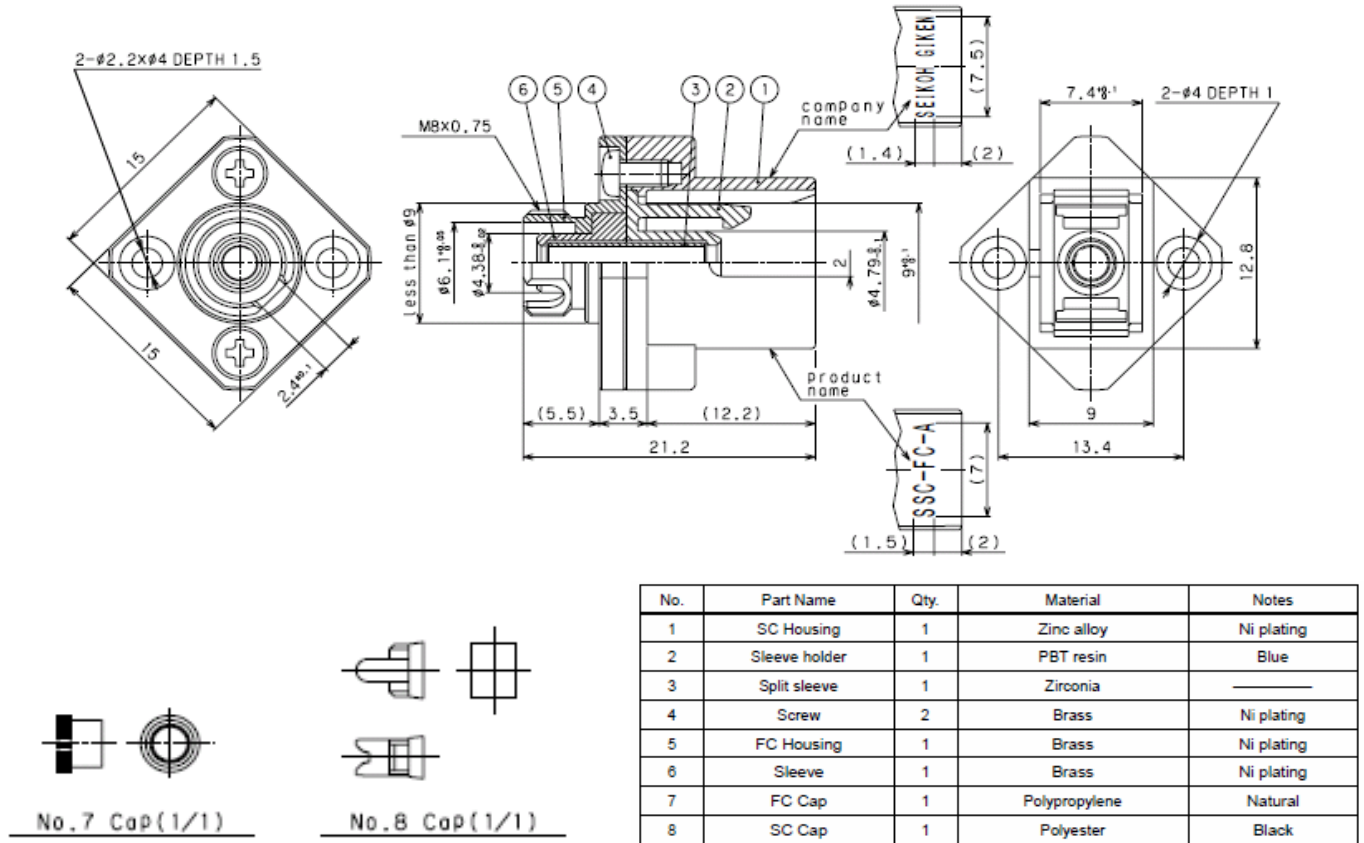
Fig. 1 Physical Dimensions
