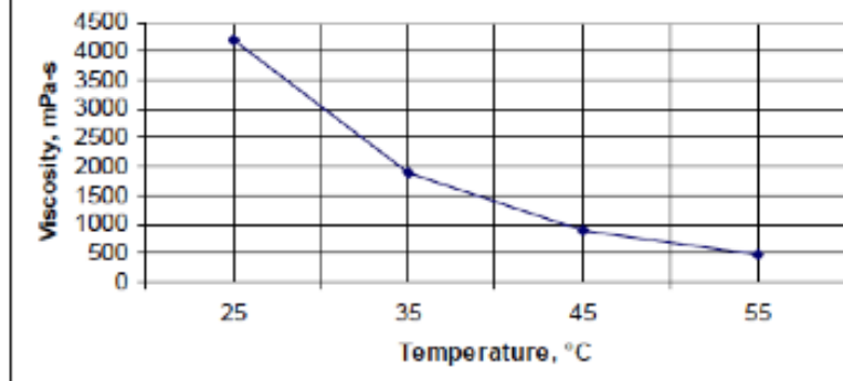
Temperature/Viscosity Curve DF-0016
