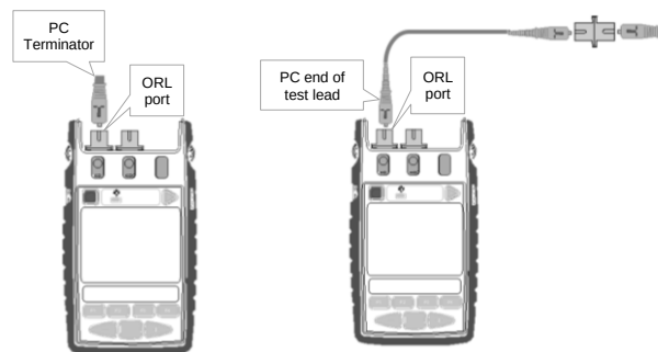
Figure 16A. Test set up for ORL verification test
