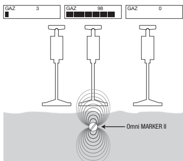
Figure 22. Signal Omni Marker II
